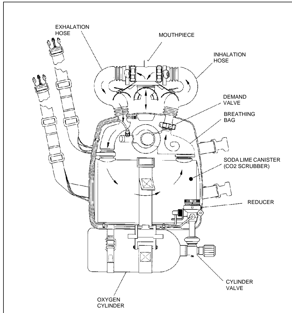
Figure 18-2. Gas Flow Path of the MK 25.
